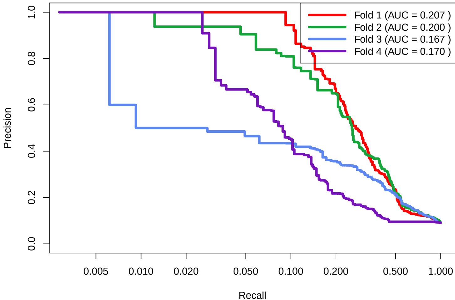
SPELL Original Datasets: 0.05 Training
